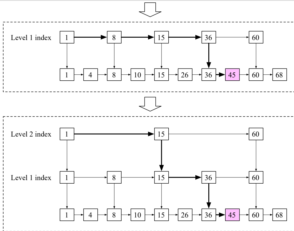
Figure 9 Skip list
