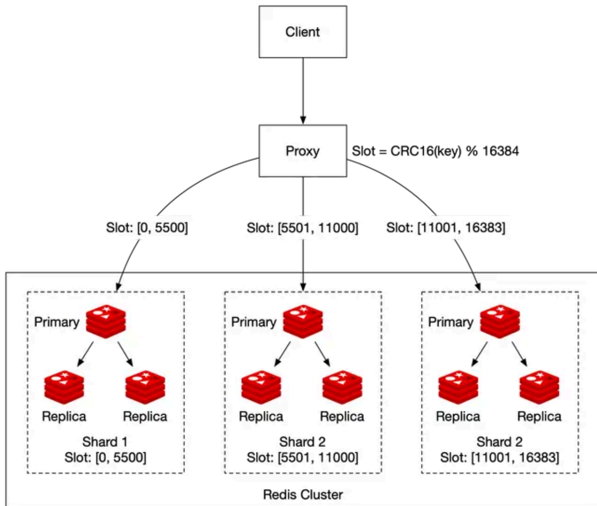
Figure 19 Hash partition
