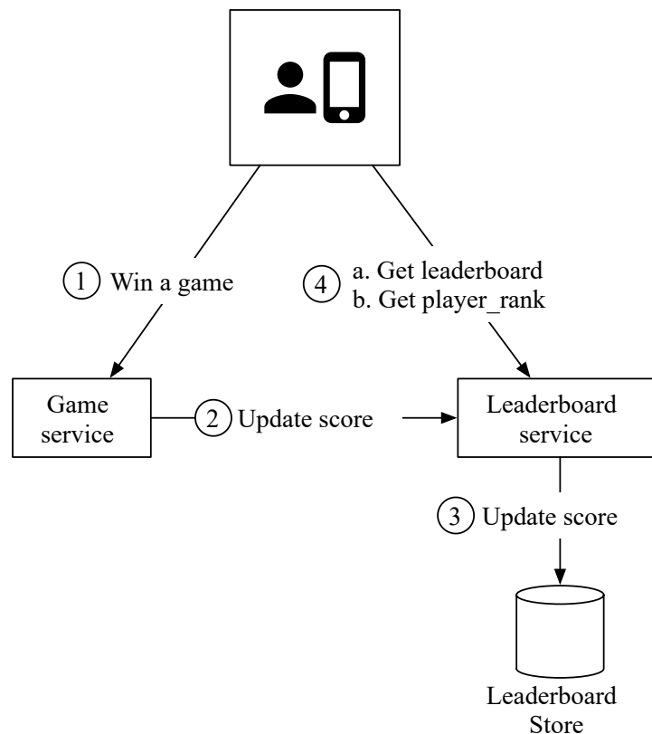
Figure 2 High-level design
