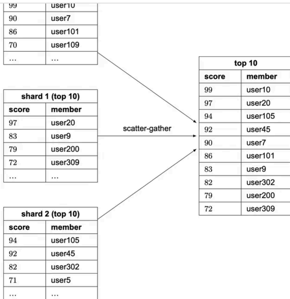
Figure 20 Scatter-gather
